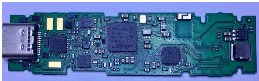
(Front of the PCB)
