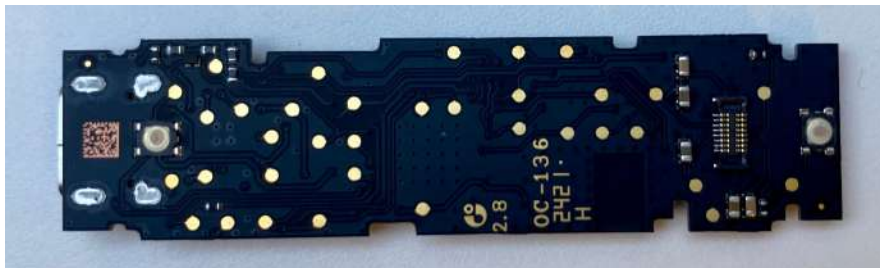
(Back of the PCB)
